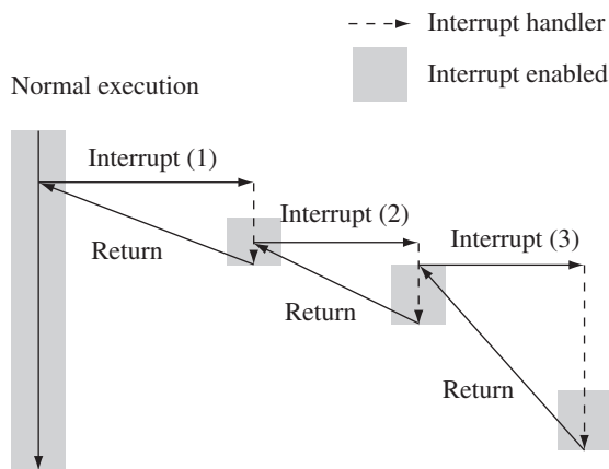
Figure 9.3 A three-level nested interrupt.
