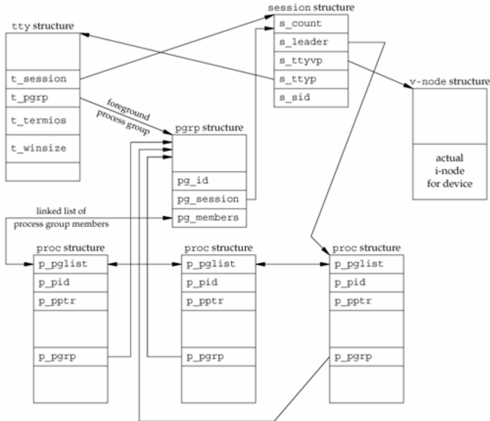
Figure 9.12. FreeBSD implementation of sessions and process groups
