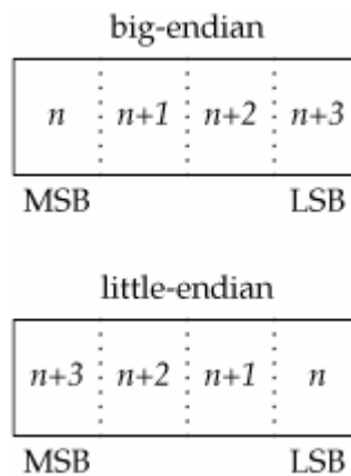
Figure 16.4. Byte order in a 32-bit integer
