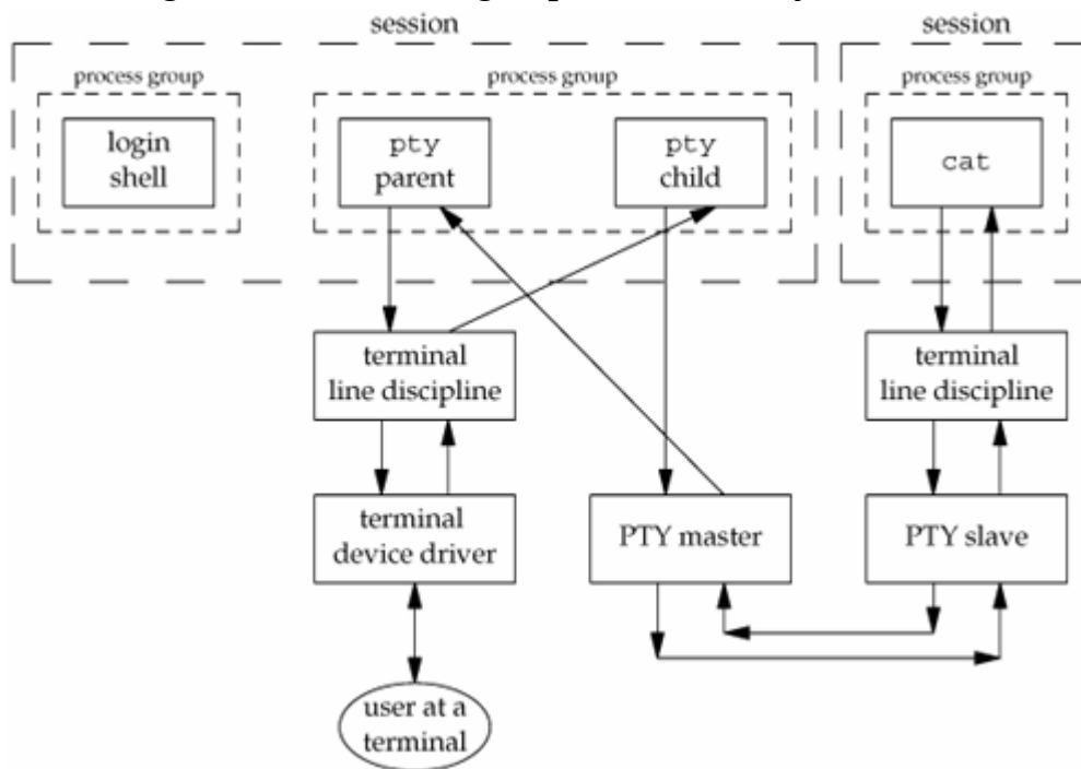
Figure 19.14. Process groups and sessions for pty cat
