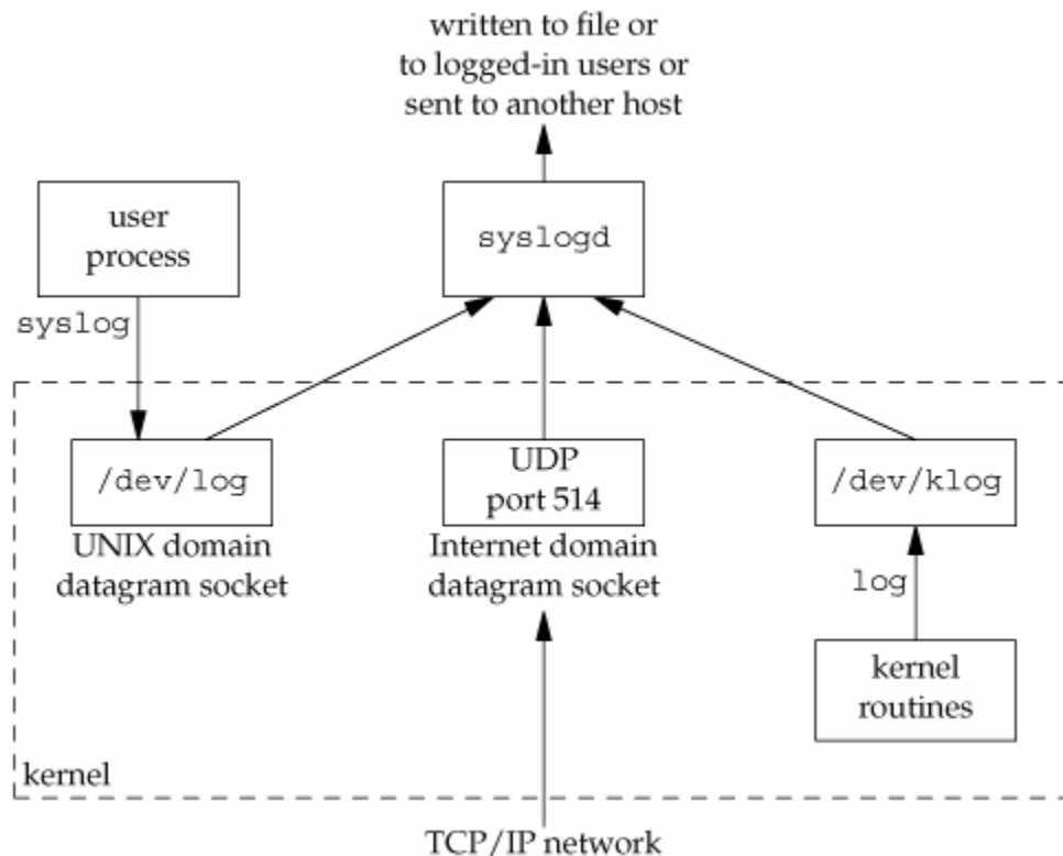
Figure 13.2. The BSD syslog facility
