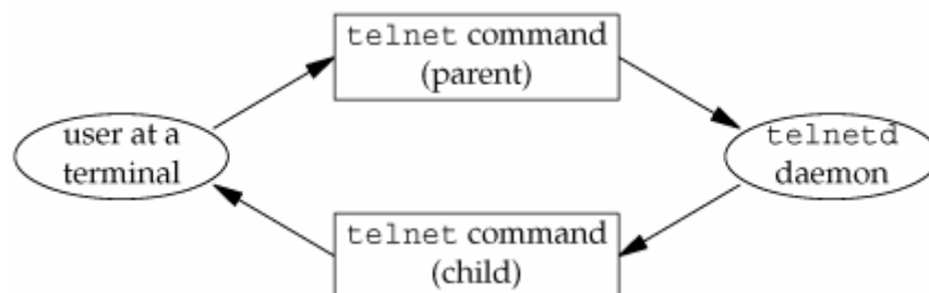
Figure 14.21. The telnet program using two processes
