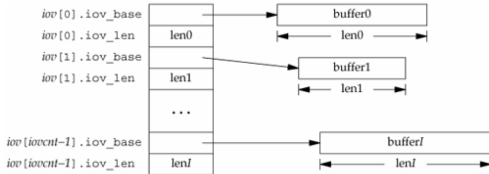
Figure 14.27. The iovec structure for readv and writev
