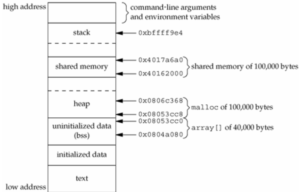
Figure 15.32. Memory layout on an Intel-based Linux system
