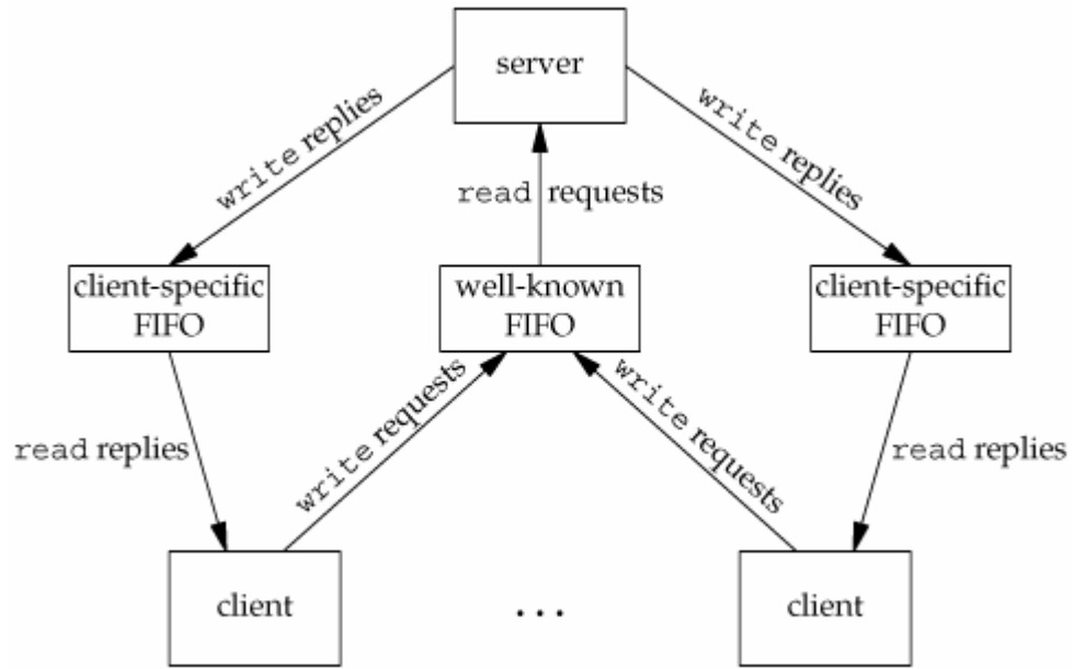
Figure 15.23. Client-server communication using FIFOs
