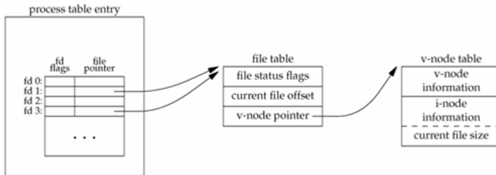
Figure 3.8. Kernel data structures after dup(1)
