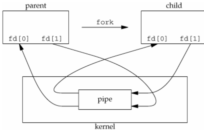
Figure 15.3. Half-duplex pipe after a fork
