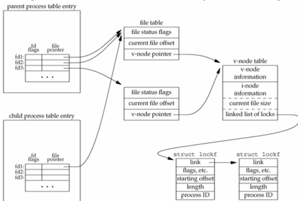
Figure 14.8. The FreeBSD data structures for record locking
