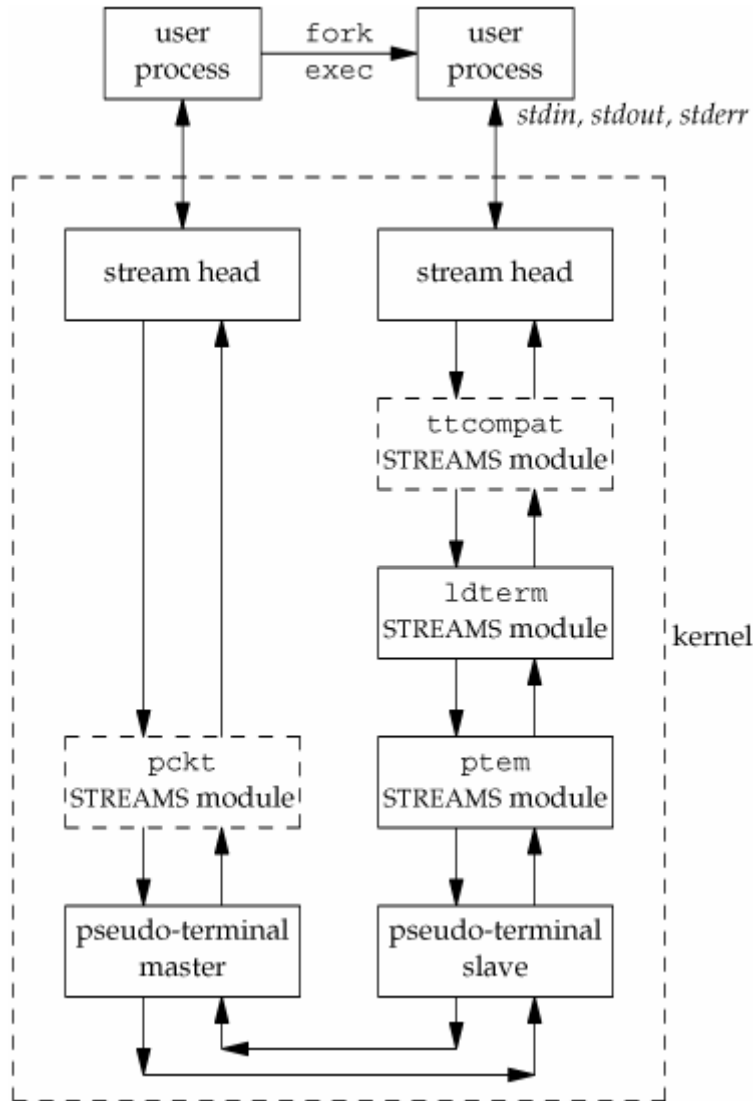
Figure 19.2. Arrangement of pseudo terminals under Solaris
