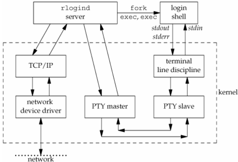
Figure 19.3. Arrangement of processes for rlogind server
