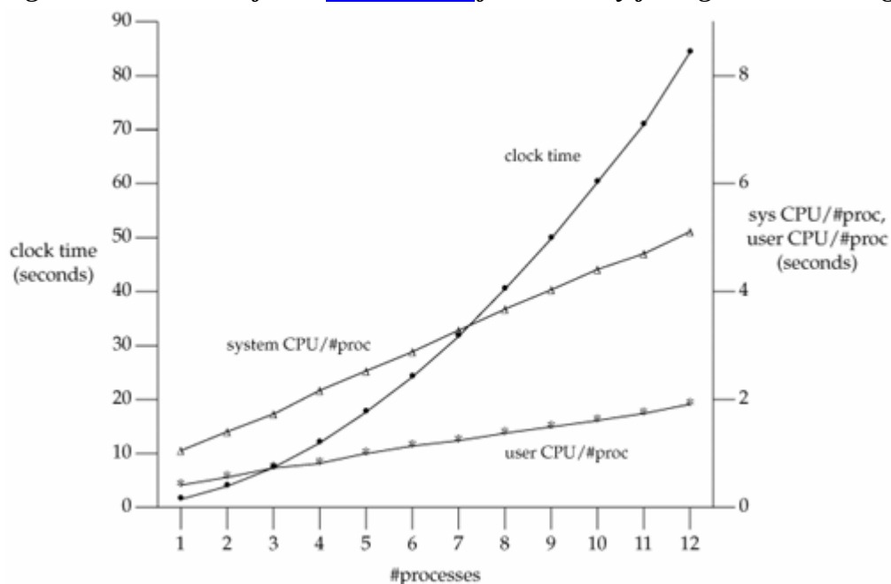
Figure 20.9. Values from Figure 20.8 for advisory fine-grained locking
