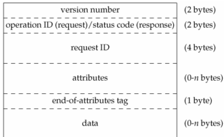
Figure 21.2. Structure of an IPP header
