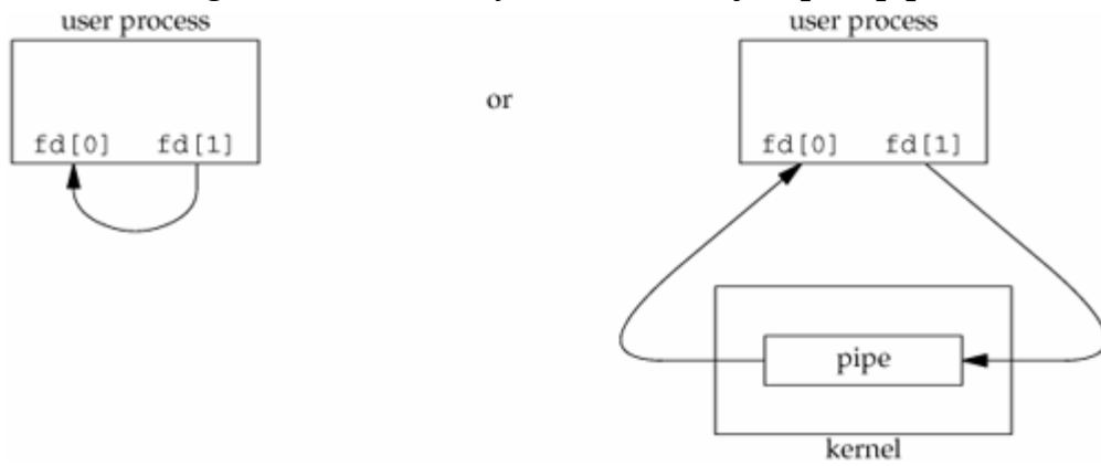
Figure 15.2. Two ways to view a half-duplex pipe
