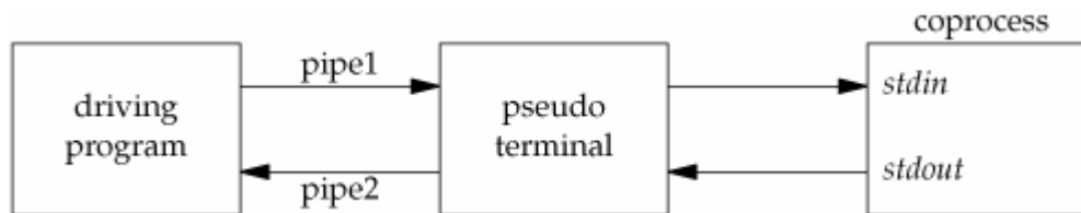
Figure 19.5. Driving a coprocess using a pseudo terminal
