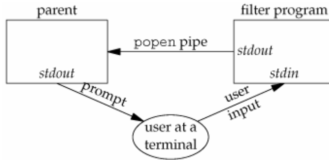
Figure 15.14. Filter to convert uppercase characters to lowercase
