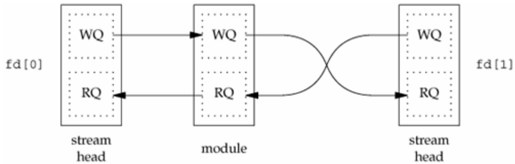
Figure 17.3. Inside a STREAMS pipe with a module
